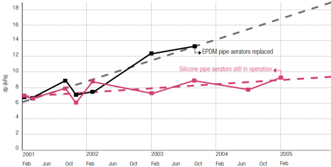
Back pressure loss across RAUBIOXON and EPDM pipe aerators under the same operating condition
